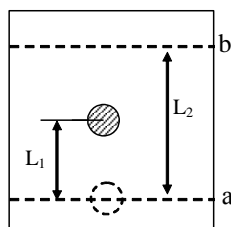
Fig. 11.2. The determination of retention index R.
