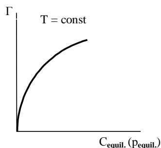
Fig.10.7. Freundlich's adsorption isotherm
