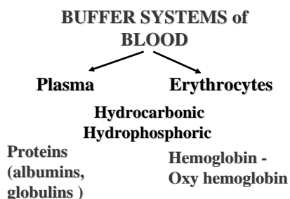
Fig. 6.2. Classification of buffer systems in blood.
