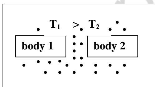
Fig. 3.2. The molecules move disorderly, collide with body 1, gain an excess of energy and then give to another molecules and at last to body 2
