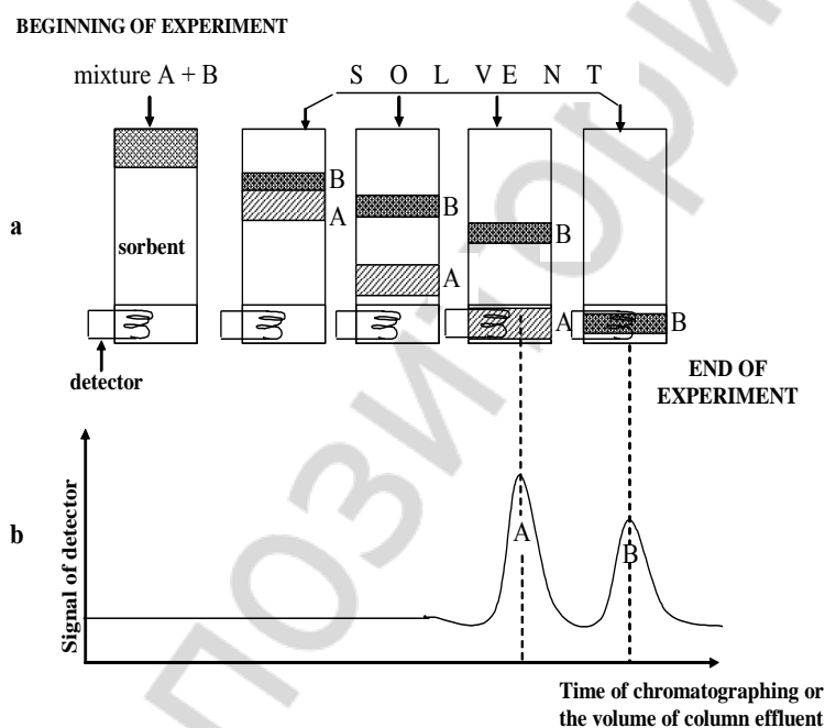
Fig. 11.3. Scheme of elution chromatography of a two-component mixture.
