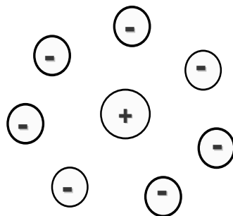
Fig. 5.5. A model of ionic atmosphere
