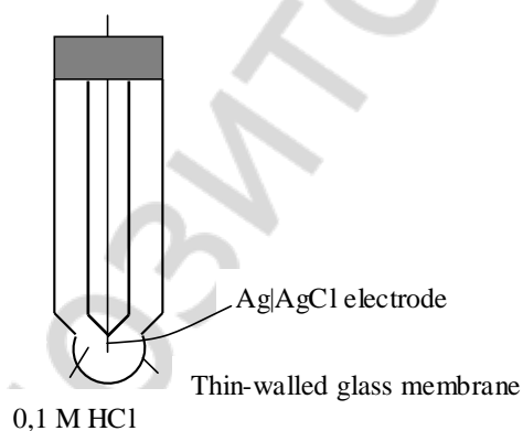
Fig. 9. 7. A glass electrode
