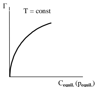
Fig.10.7. Freundlich's adsorption isotherm
