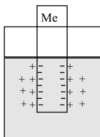
Fig.9.4. Double electric layer at the interface 'metal-solution'
