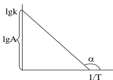
Fig. 4.5. The relationship between \lg k and 1/T
