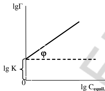
Fig.10.8. Graphic estimation of constants in Freundlich's equation
