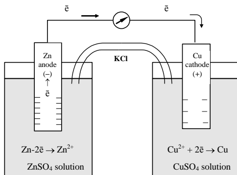
Fig. 9.5. Jacobi-Daniell galvanic cell
