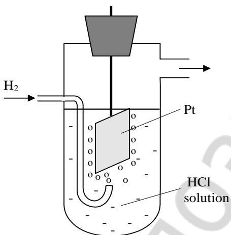
Fig.9. 6. Standard hydrogen electrode
