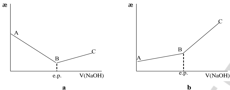
Fig. 9.3. Conductometric titration curves
