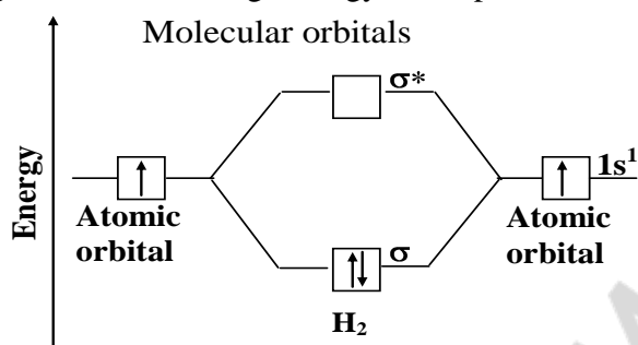
Fig. 2.11. Bonding and antibonding molecular orbitals in H 2
