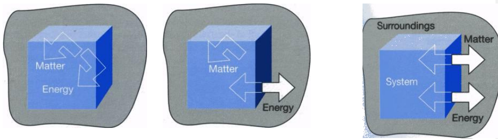
Fig. 3.1. Thermodynamic systems
