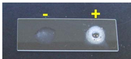
Figure 6.4 - Catalase detection
