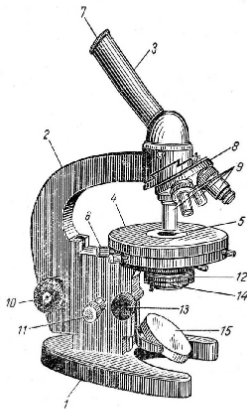
Fig. 1. The structure of a light microscope:
